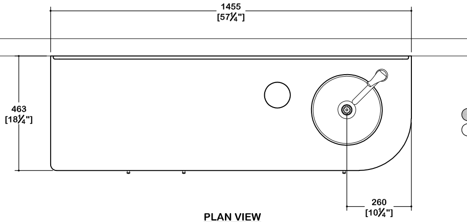
PLAN VIEW
